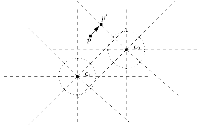
Figure 2: Computing the coreset.
