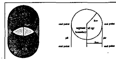
Fig. 5. Computing A(s|Lss)
