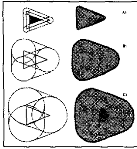
Fig. 6. Computing A(cgr|Lss)
